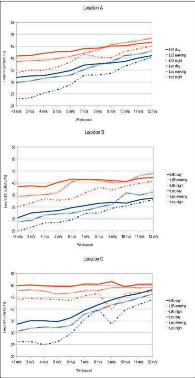
Figure 4: Measured L_{95} and L_{eq} in dB(A,LF)
