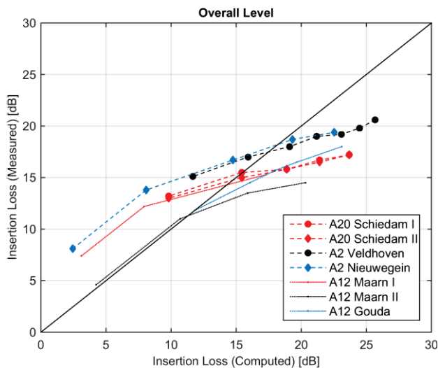
Figure 5. Insertion loss, measured vs. computed
