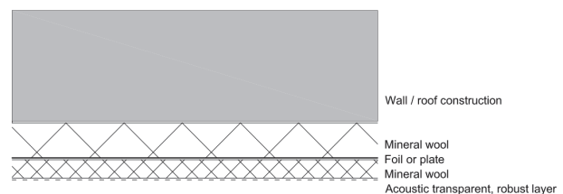
Figure 2. Example of a broad band absorption material.
