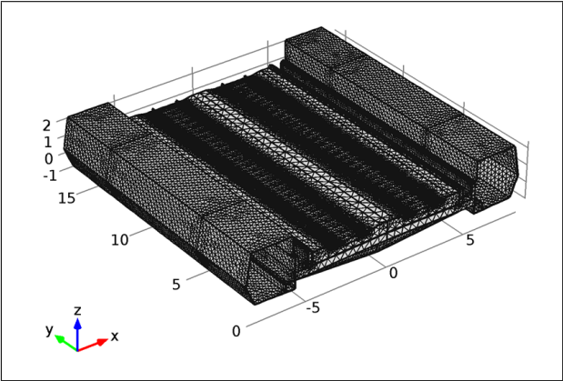
Figure 10. Mesh of the new bridge for a frequency of 100 Hz
