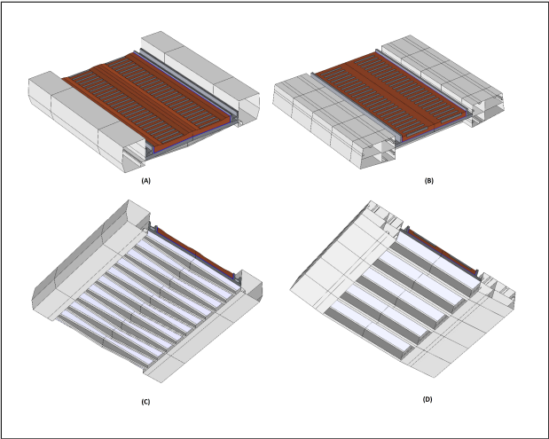
Figure 9. Top and bottom view of the 3D-models of the new bridge (A & C) and the reference bridge (B & D)
