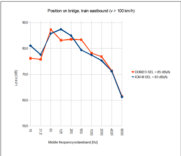
Figure 8. Spectral values of SEL at location 1 near the reference bridge for two types of trains
