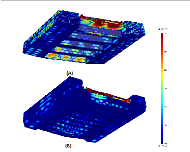
Figure 11. Vibration velocities ( L_v ) for an excitation of 1 N at a frequency of 141 Hz for the reference bridge (A) and the new bridge (B)
