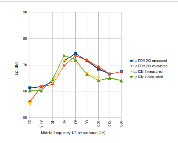
Figure 12. Comparison of calculated and measured bridge noise level at 35 m from the nearest track of the reference bridge
