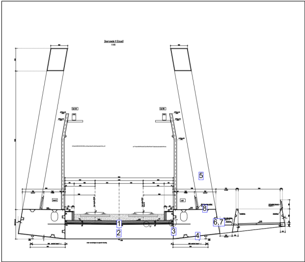
Figure 5. Location of the accelerometers on the reference bridge (cross-section).
