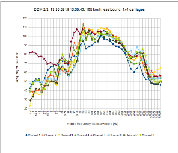
Figure 6. Spectral vibration acceleration of the passage of a train at eight locations on the reference bridge.
