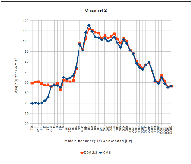
Figure 7. Spectral vibration acceleration at location 2 on the reference bridge for two types of trains.
