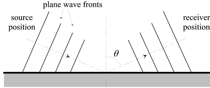
Figure 1: Reflected-sound path for plane wave sound transfer.
