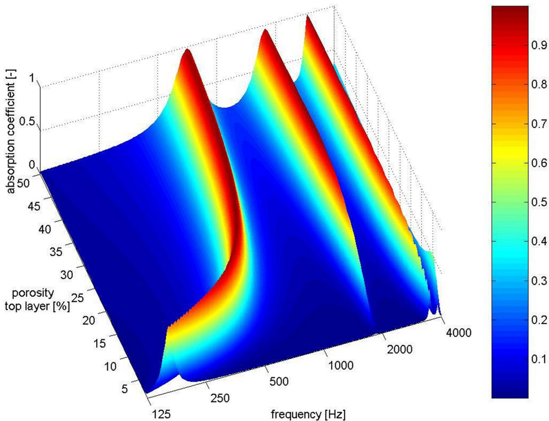
Figure 4: Absorption spectrum as a function of the top layer porosity for road 2L-coarse.
