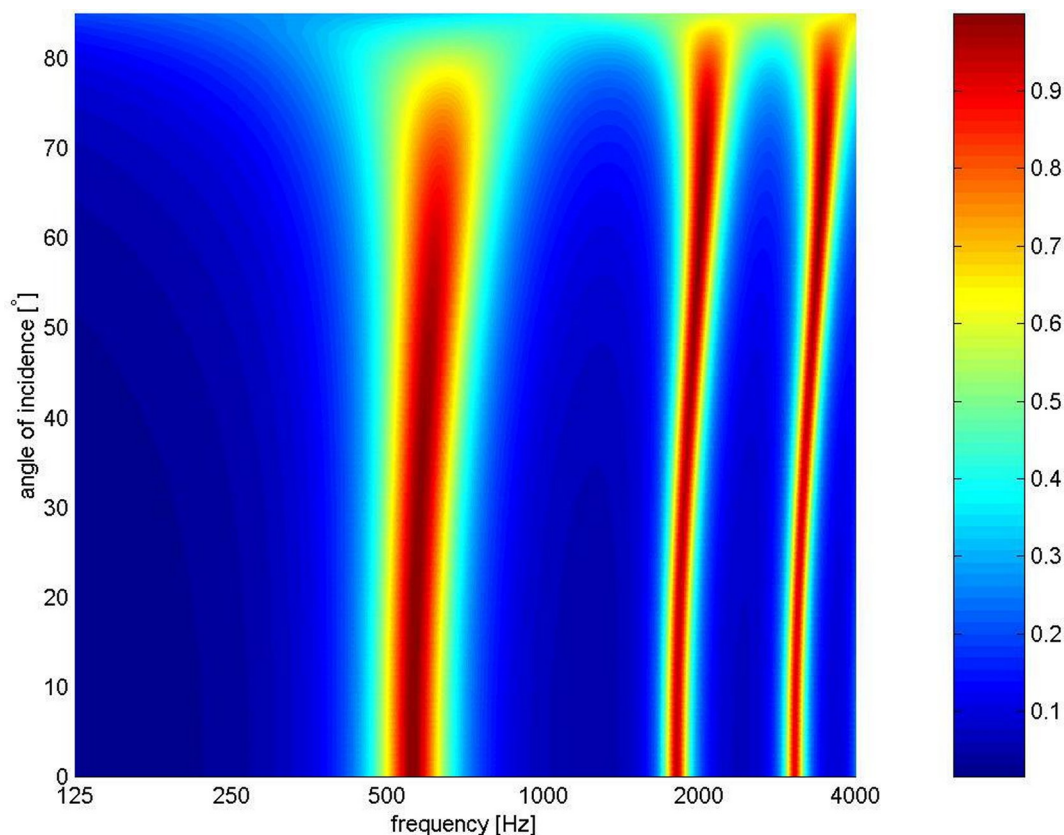
Figure 2: Absorption spectrum as a function of the angle of incidence for road 2L-coarse.
