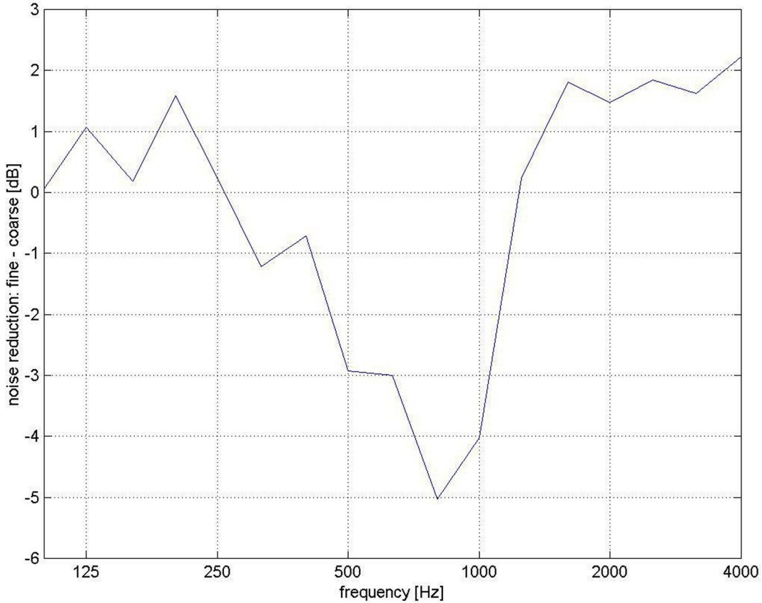
Figure 5: Measured effect of finer texture of the two-layer porous asphalt on the tyre/road noise.
