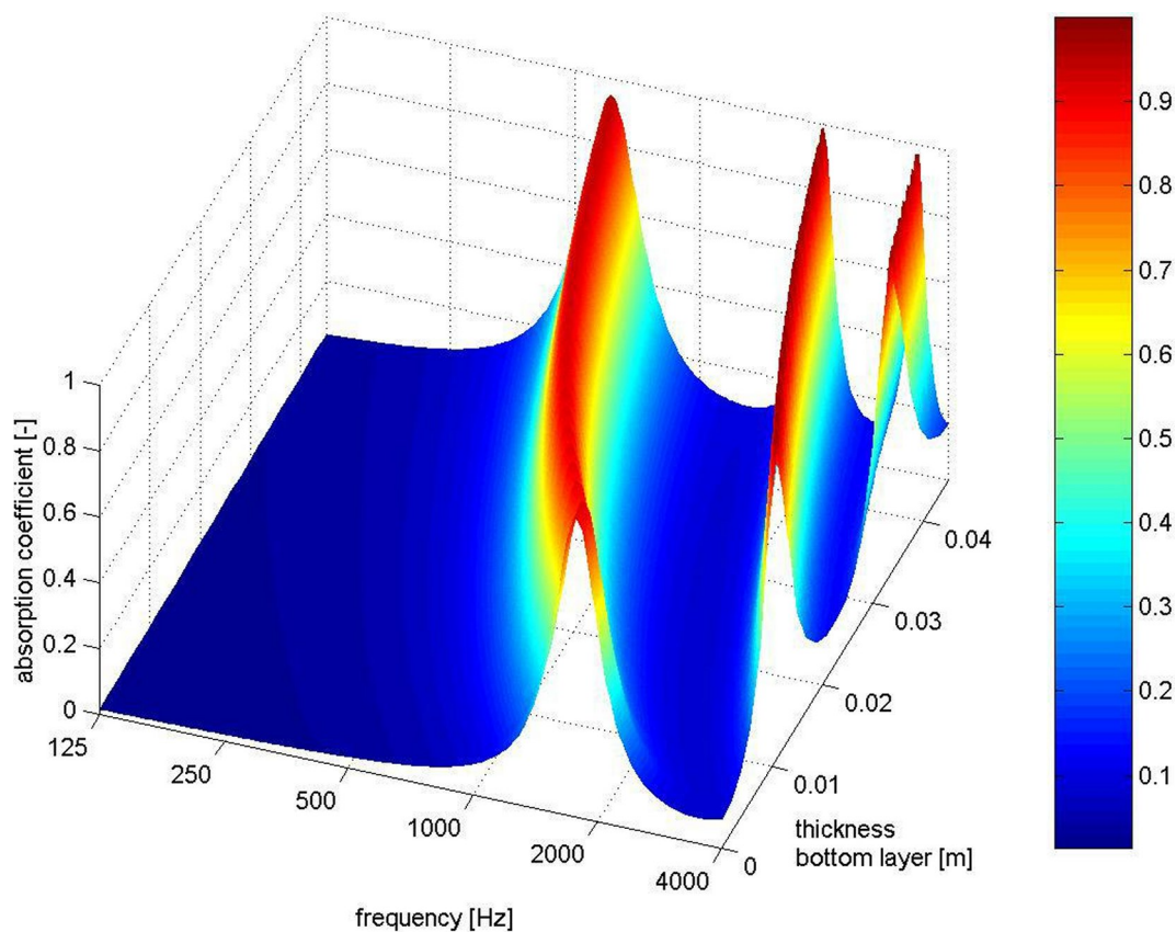
Figure 3: Absorption spectrum as a function of the bottom layer thickness for road 2L-coarse.
