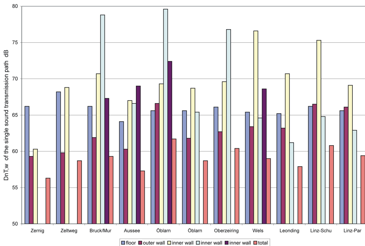
Figure 4: D_{nT,w} -values for the different single sound transmission paths rooms one above the other.
