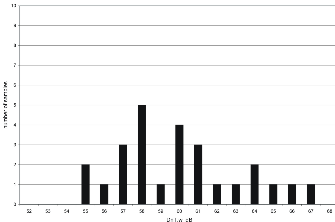
Figure 1: Weighted standardised sound level difference between adjacent rooms.
