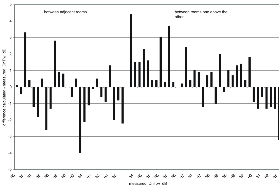
Figure 5: Difference between the calculated and the measured D_{nT,w} -values.
