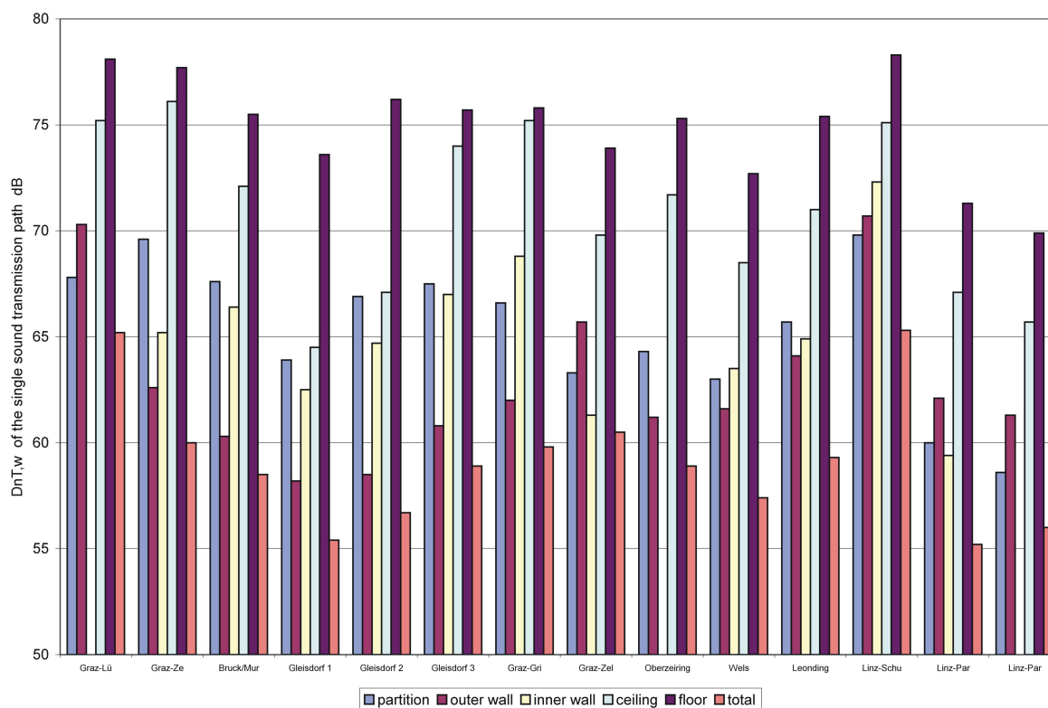
Figure 3: D_{nT,w} -values for the different single sound transmission paths adjacent rooms.
