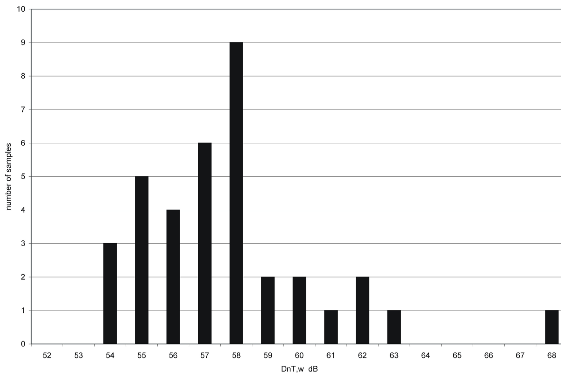
Figure 2: Weighted standardised sound level difference between rooms one above the other.
