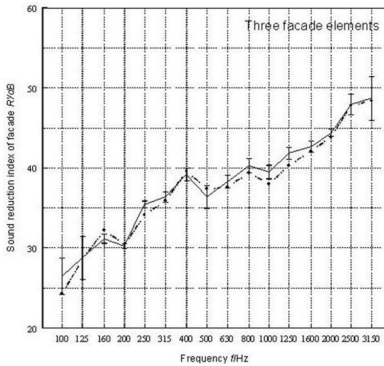
Figure 2: Variation in sound insulation, combination (1, 5, 6).
