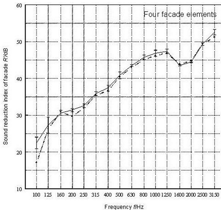
Figure 1: Variation in sound insulation, combination (1, 3, 6, 8).
