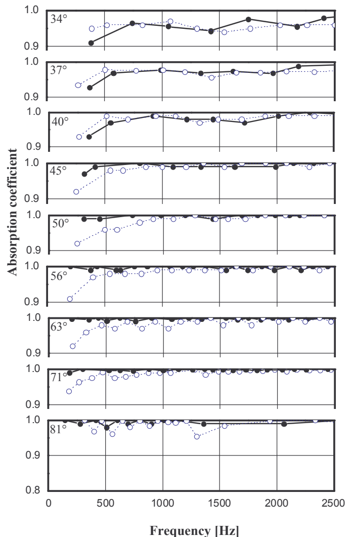
Figure 4: Absorption coefficient of ASA (●) and BCA (○) for different angles of incidence.
