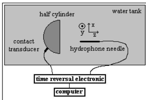
Figure 1: Top view of the experimental setup. The contact transducer is fixed to the duralumin half-cylinder and the hydrophone needle is moved in a 3D domain
