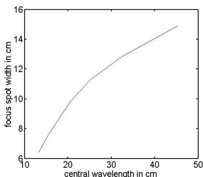
Figure 6: focal spot width versus the central wavelength
