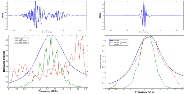
Figure 4: Top: left: the focusing signals E to be emitted from array 1 to focus on array 2, calculated by IF; right: the resulting signals F obtained on array 2. Bottom: their fourier transforms: left, the fourier transform of the signals E (red, dash-dotted), to be compared to the signals E computed by transmission TRM (green, dashed) and target (blue, plain); right, the spectras of the subsequent focalisation F (red, dash-dotted), with TRC (green, dashed) and target signal (blue, plain).
