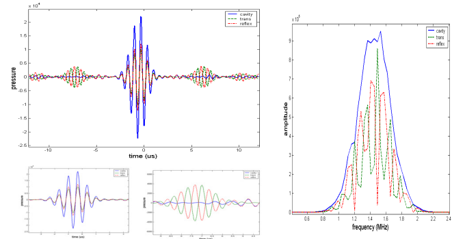
Figure 3: Temporal shape (left) and spectrum (right) of the signals received on array 2 after time-reversal processes. Plain, blue: TRC (using both arrays 1 and 2). Dashed, green: TRM in transmission (using only array 1). Dash-dotted, red: TRM in reflexion (using only array 2). The two insets on the left represent the main wavefront (left) and the first preceding echo (right)
