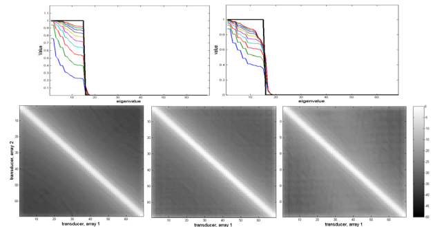
Figure 5: Top: progression of the eigenvalues of H M_n , for simple iteration method (left) and double iteration method (right). The thin, colored curves correspond to the value of the eigenvalues, for iteration orders from 1 to 10. They converge towards the black, thick line, showing the values of the eigenvalues of the H H^{-1} of the IF. Bottom: The images of H M_{10} , calculated by simple iteration method (left), H H^{-1} of the IF (center), and H M_{10} , and double iteration method (right).
