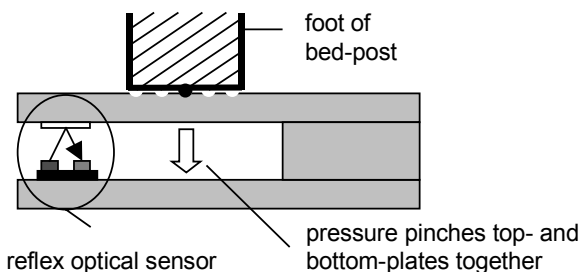
Fig 1: Schematic drawing of a sensor (side view)
