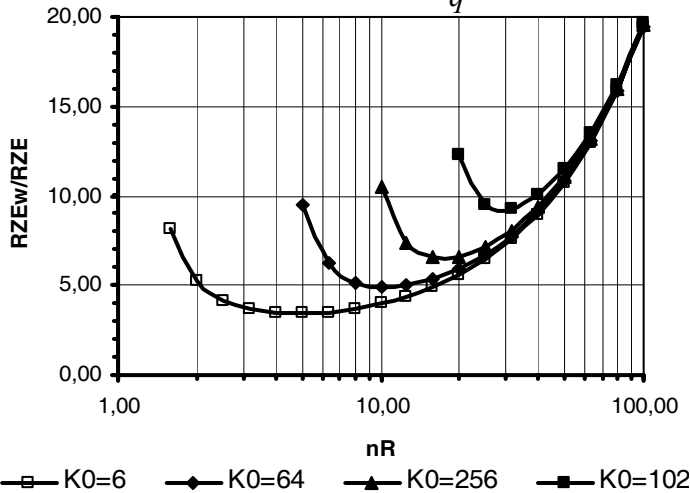
Figure 3: computation time in CTU for finding the next wall as a function of the degree of quantization n_r = n_q with the voxel crossing technique according equ.16; parameter K_0 = number of walls; to be compared with K_0 CPU = constant for non-accelerated ray tracing
