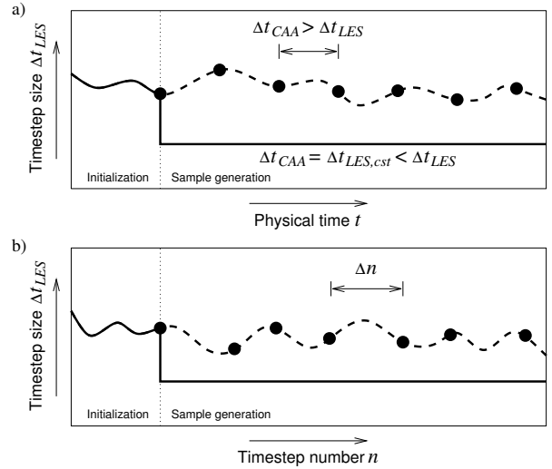
Figure 4: Timestep \Delta t_{LES} as a function of physical time t (a) and of timestep number n (b) for two different coupling strategies.
