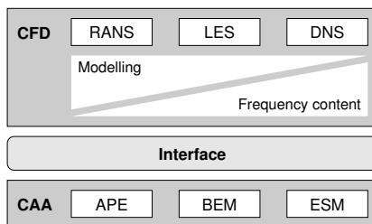
Figure 1: Coupling of CFD with CAA.
