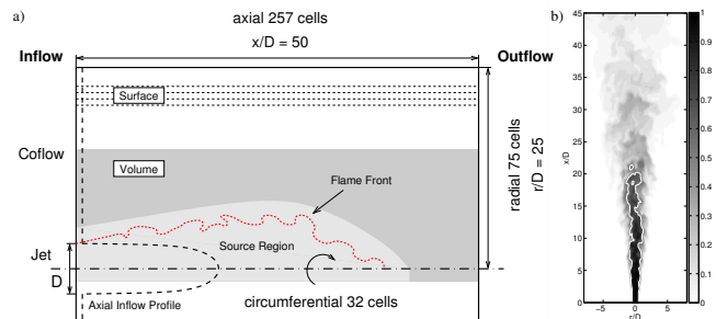
Figure 2: (a) Sketch of the configuration and the computational domain. (b) Instantaneous snapshot of the mixture fraction field.
