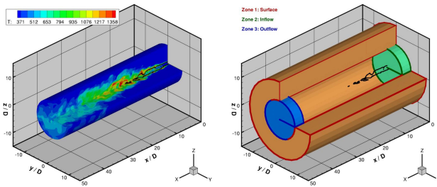
Figure 3: Interface domains for CAA methods. Left: Volumetric domain for APE, colored by the instantaneous distribution of T in Kelvin – Right: Surface domain for BEM & ESM.
