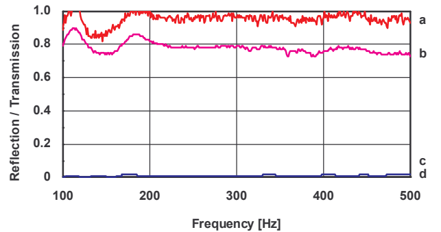
Figure 3: Transmission coefficient \tau of the empty duct (—, a) and of a fabric sample (—, b); Reflection coefficient \rho of the empty duct (—, c, straight line at 0) and of a fabric sample (—, d).
