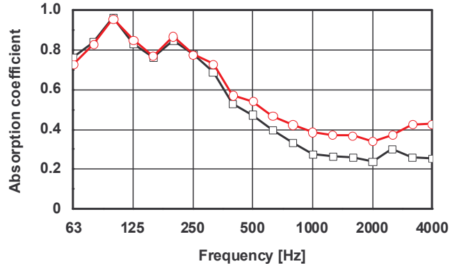
Figure 4: Absorption coefficient \alpha_s of Compound Panel Absorbers without ( \square ) and with ( \circ ) a fabric cover.
