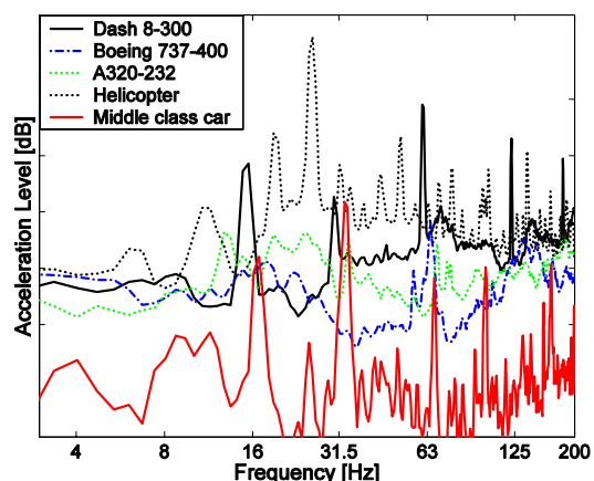
Figure 2: An overview of vibration exposure in passenger cabin for different transport facilities (aircraft, helicopter and vehicle).
