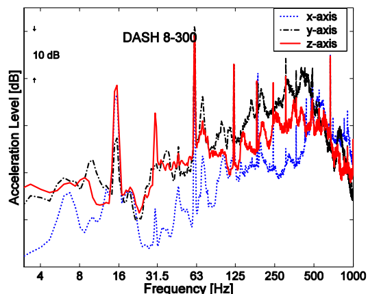
Figure 1: Typical averaged vibration spectra of a DASH 8-300 during cruise condition in all three (x-, y- and z-) directions. The vibrations were measured at the seat rail of seat F in row 12.
