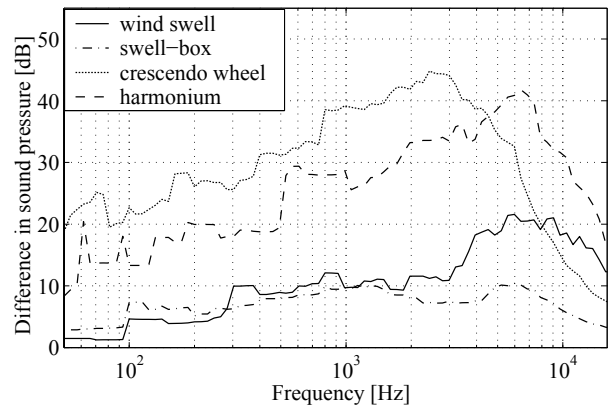
Figure 2: Spectral differences between the lowest and the loudest setting for different expression devices (wind swell, swell-box and crescendo wheel). Each curve shows the average over several instruments measured as described in the text. All values were calculated from differences in the octave band spectrum.
