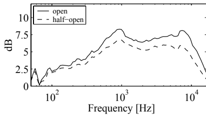
Figure 1: Spectral difference between the open and the closed door setting of the swell box (solid line), and the spectral difference between the half-open and the closed door setting (dashed line). Here, the transfer function between a loudspeaker placed in the swell-box and the left ear of a dummy head is shown.
