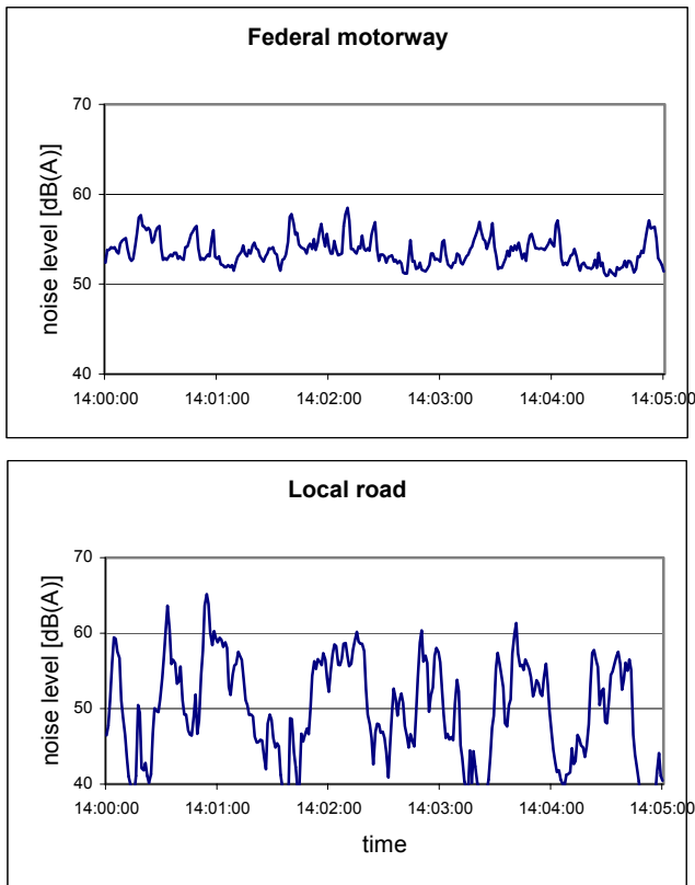
Figure 1: Short-time noise-time patterns of a federal motorway at larger distance and a local rod
