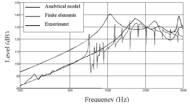
Figure 5: acoustic pressure radiated by the PVDF loudspeaker at 5 mm from the dome centre for a 10 V rms voltage. Back pressure = 50 mBar, Film thickness = 25 microns.
