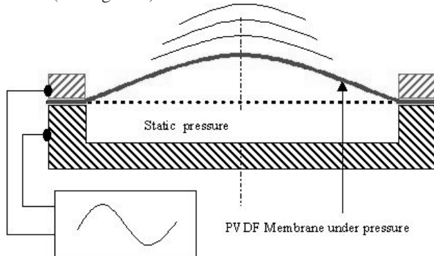
Figure 1: PVDF loudspeaker principle. The dome shape is obtained by means of a static back pressure. The radiated acoustic pressure is produced by a time variable voltage.
