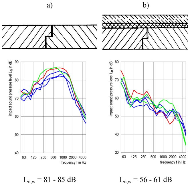
Figure 2: impact sound pressure level of timber floors
