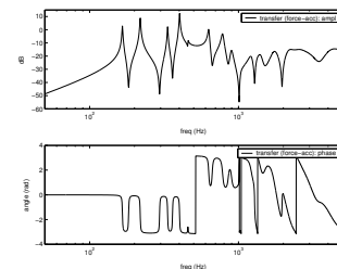
Figure 2: Plant transfer function between the structural actuator and the accelerometer.
