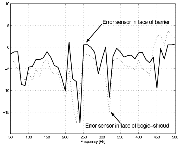
Figure 4: Measured reduction of the mean squared pressure at reference point ( x=2.1m , y=1m ), The secondary source and the reference sensor at the bogie-shroud; The secondary source and the reference sensor at the barrier
