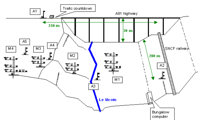
Figure 1: The monitoring site of Saint-Berthevin (F) – “A” stands for acoustical mast and “M” for meteorological mast.
