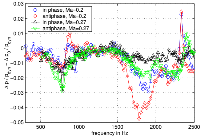
Figure 4: Change of pressure drop depending on incident sound for the rectangular duct section. \circ fundamental and \diamond antisymmetric mode for u = 69 \text{ m/s} , \triangle and \nabla for u = 93 \text{ m/s} respectively.
