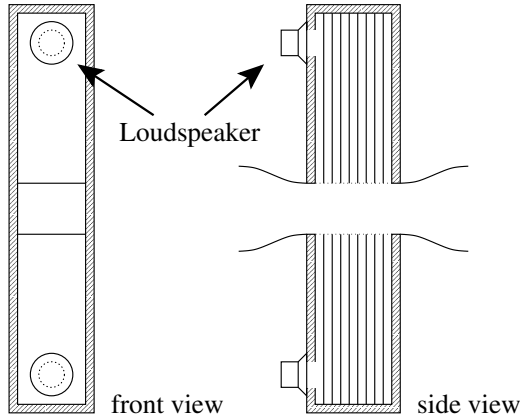
Figure 3: Yielding-walled duct section with accelerated flow
