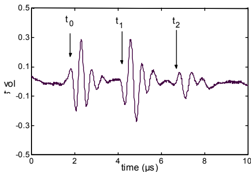
Figure 2: Echoes from the basis of a rod made of duralumin with a radius of 0.4mm, immersed in glycerine ( C=1.92\text{mm}/\mu\text{s} )
