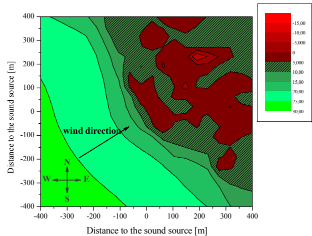
Figure 1: Excess attenuation in dB caused by perfectly reflecting surface influence on the sound propagation in comparison to a completely absorbing surface. Positive values: decreasing sound immission, negative values: increasing sound immission, zero: no surface influence
