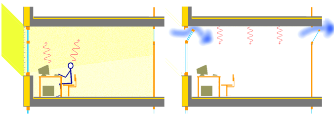
Figure 1: The basic concept of passive cooling - an office room shown as an example. During day (left) the room is heated by several sources: the sun, electric light, computers and other equipment, and the occupants. Part of this heat is stored into the massive concrete ceiling. During night (right) the room is vented by cool night air and the heat is unloaded from the ceiling. For good cooling effect the storage element (the ceiling) must show a large surface to the room at good thermal conductivity and high storage capacity. This prohibits acoustic absorbers covering the ceiling.
