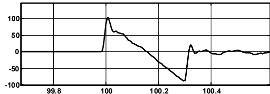
Figure 1: Example of a Mach wave (N wave) in the vicinity of a small projectile trajectory.
