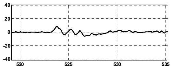
Figure 2: Example of a muzzle wave due to a small arm weapon at large distance.
