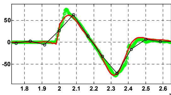
Figure 6: N wave measured with the cavity microphone and reconstructed (red solid line) and measured with an external microphone (line with green circles, sampling rate 200 kHz, line with black circles sampling rate 12 kHz).
