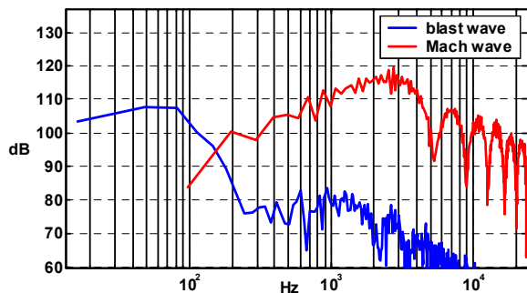
Figure 3: General spectral components of (a) Mach wave and (b) muzzle wave.
