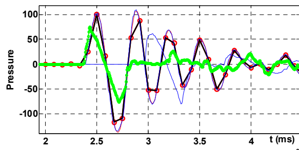
Figure 5: N wave measured with an external microphone up to 100 kHz (green solid line) and measured with the cavity microphone (line with red circle, sampling rate 12 kHz).
