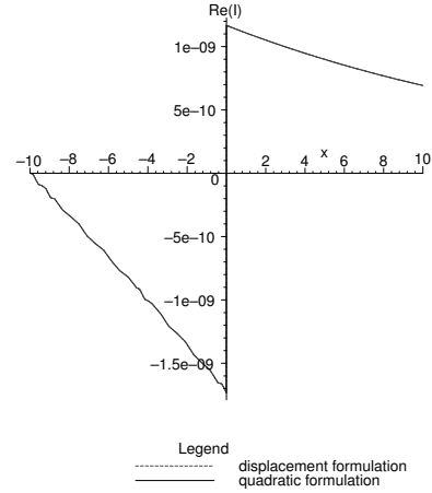
Figure 4: Real part of the structural intensity.
