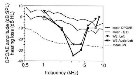
Figure 4: high-resolution audiogram (squares) vs. DPgram (triangles) in an ear with noise-induced hearing loss. The DPgram is conventionally plotted for the 2f_1-f_2 DPOAE referred to frequency f_2 along the horizontal axis. The thin, almost parallel lines delineate the area where normal DPOAEs should fall. The dashed line marks the limit of background noise.
