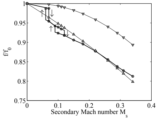
Figure 3: Variation of screech frequency f with the secondary Mach number M_s and comparison with analytical formulæ. NPR = 3.17. D_s = 200 mm. \nabla Bryce & Pinker [1], \triangle Tam [14], \circ present study, increasing M_s , \square present study, decreasing M_s . f_0 is the computed or measured frequency without flight effect : \nabla and \triangle : 3588 Hz, present study 3210 Hz.
