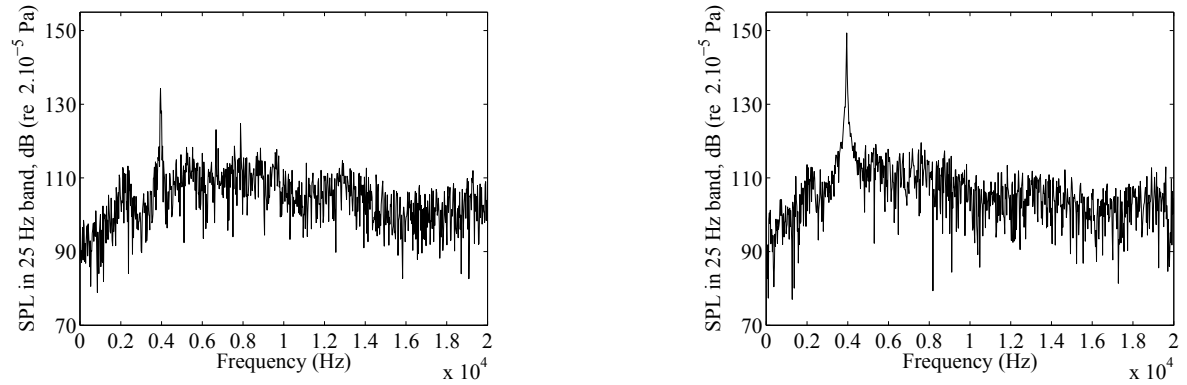
Figure 6: Time frequency analysis of the unsteadiness of mode B (see Fig. 5 right). \text{NPR} = 2.54 . Left, sound pressure level (SPL) of a weak screech section from 0.046 s, 4096 values long. Right, SPL of a strong screech section from 0.84 s, 4096 values long.
