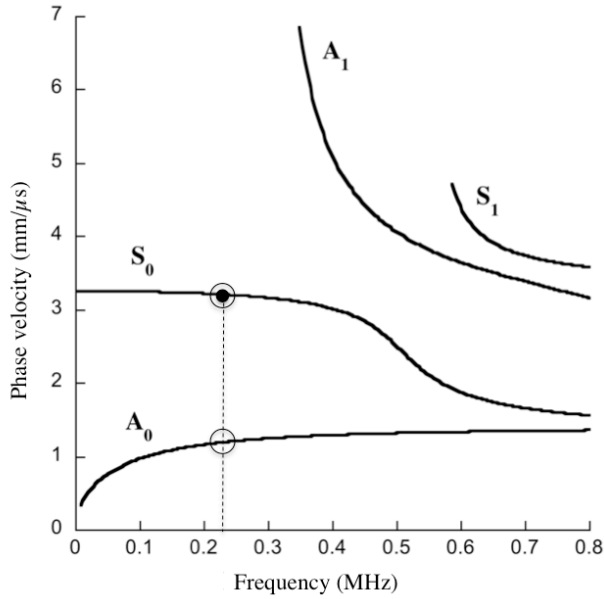
Figure 3: Dispersion curve for 2.36mm thick Carbon epoxy composite plate with operating points, incident wave (●) and scattered waves (○).
