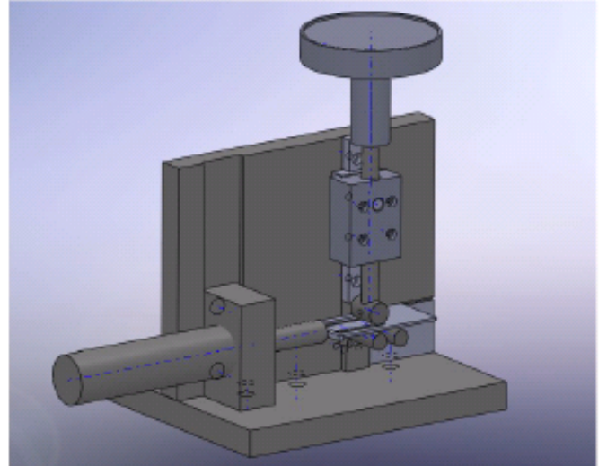
Figure 2: Scheme of the experimental bench.
