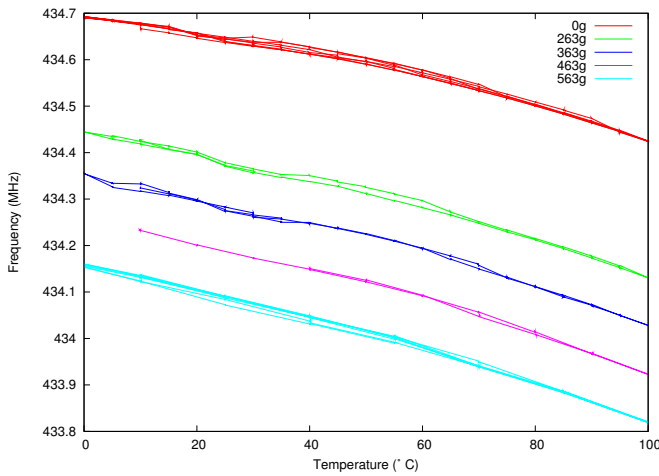
Figure 5: Absolute frequency shift with temperature for different mass loading.
