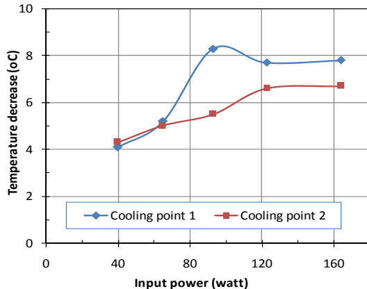
Figure 6. The temperature decrease for various input electric power.
