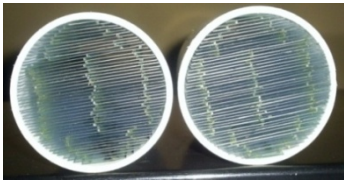
Figure 2. The cross section of the parallel plate stacks. The stack's housings are 2 in. PVC pipe.
