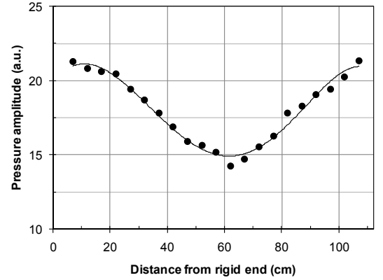
Figure 3. The relative pressure amplitude distribution in the resonator tube.
