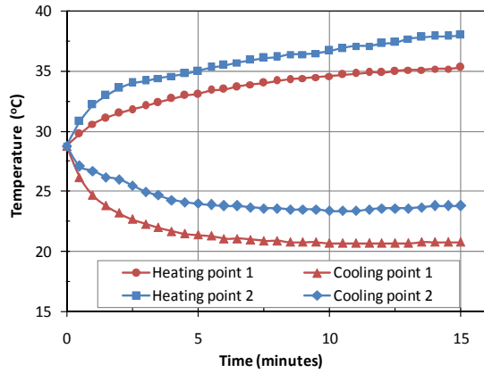
Figure 4. Temperature changes in time of the cooling and heating points 1 and 2 at frequency of 147 Hz and input power of 90 W.
