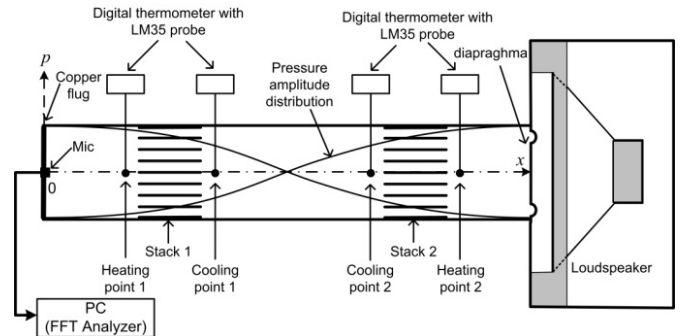
Fig.1 The schematic diagram of the thermoacoustic cooling system with two stacks in a half-wavelength resonator tube.
