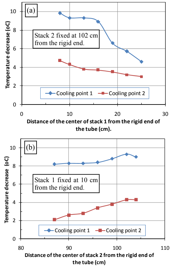
Figure 7. The temperature decrease: (a) for various location of stack 1 (stack 2 fixed at 102 cm from rigid end), and (b) for various location of stack 2 (stack 1 fixed at 10 cm from rigid end).
