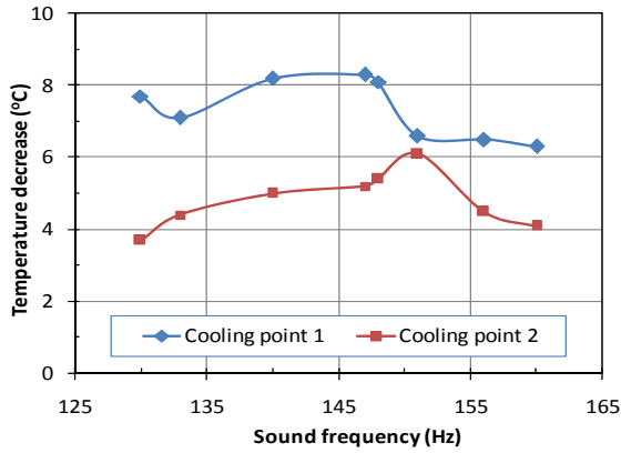
Figure 5. The temperature decreases for various sound frequencies.
