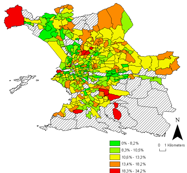
Figure 2: Spatial variability of potential noise exposure on road traffic L_{den} (%)
