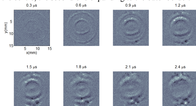
Figure 5: Space-time signals recorded for the sensor with ring geometry electrodes.
