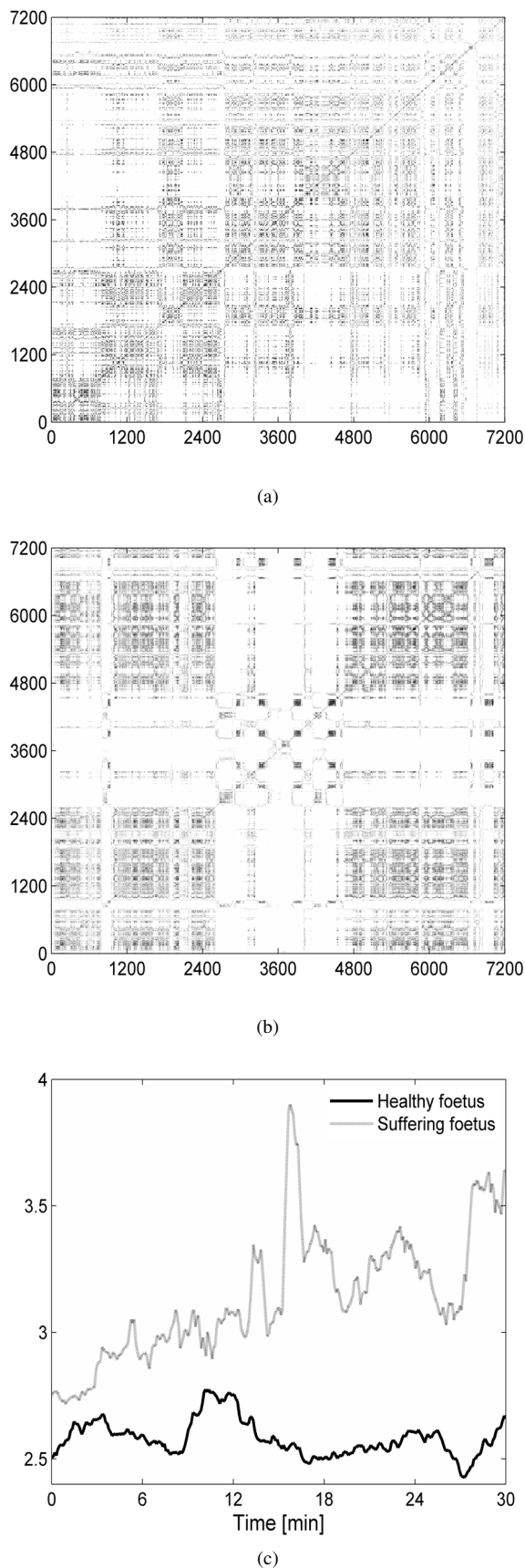
Figure 5: The RP matrix computed for: (a) a healthy foetus and (b) a suffering foetus. Figure (c) presents the mean diagonal distance computed in a sliding window manner with a window of three minutes.
