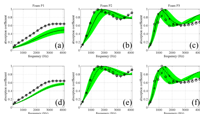
Figure 3: Sound absorption coefficient of 1 in. thick polyurethane foam layer: ((a),(d)) foam P1, ((b),(e)) foam P2, ((c),(f)) foam P3; (thick continuous line) model using the estimated non-acoustic properties from strut measurements; (thick discontinuous line) model using the estimated non-acoustic properties from cell size measurement; (green area) propagation of microstructure measurements uncertainties; (O,+) impedance tube measurements.
