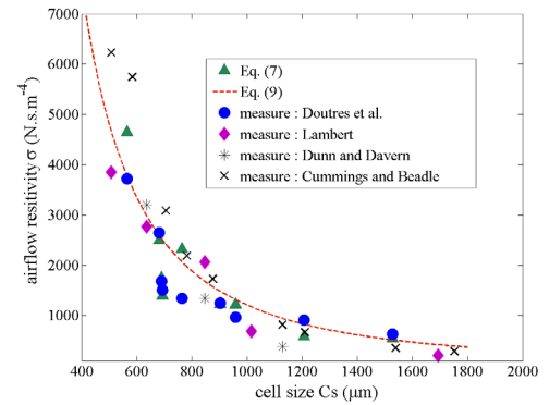
Figure 2: Airflow resistivity versus cell size for fully reticulated polyurethane foams ( R_w=100\% ). Eq. (7) uses measurements of strut length and thickness; Eq. (9) uses measurement of cell size only.
