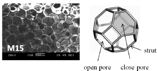
Figure 1: SEM picture of the partially reticulated polyurethane foam M15 and shape of the unit cell (PUC).
