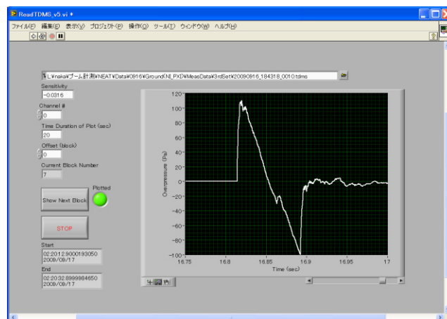
Figure 5: Instrumentation graphical user interface of outdoor recorded sonic boom.
