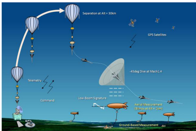
Figure 13: Diagram of D-SEND #2 test planned for 2013.
