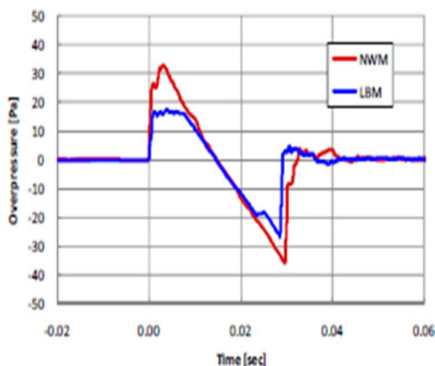
Figure 11: Contrasting sonic boom signatures recorded with NWM and LBM test bodies.
