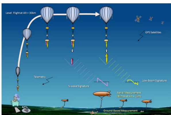
Figure 9: Diagram of drop test #1
