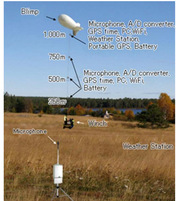
Figure 7: Outdoor measurement systems.
