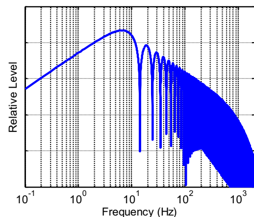
Figure 1: Acoustic content of a sonic boom.
