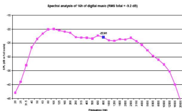
Figure 4 Spectrum of real-world music samples
