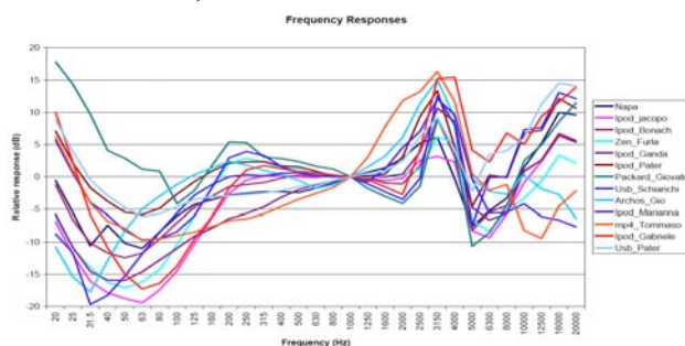
Figure 11 – Frequency response curves
