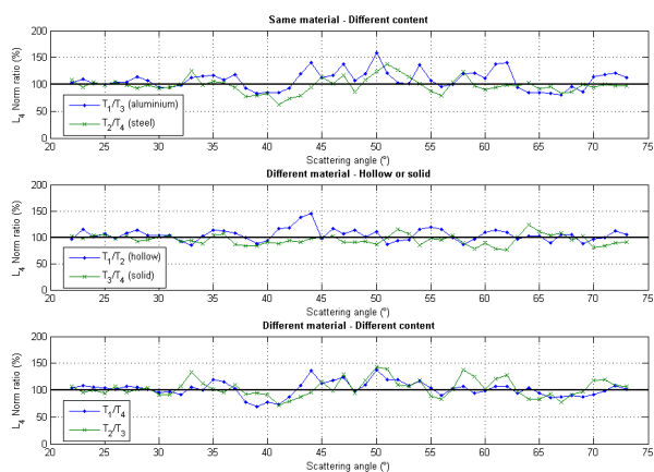
Fig.3 Variations of the L^4 norms of signals scattered by targets placed proud on silt. The thick black line shows the 100% level, i.e. when the targets have the same response.
