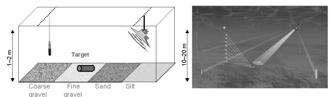
Fig.1 Scaled tank experiments (left) were used in preparation for full-scale sea trials (right).
