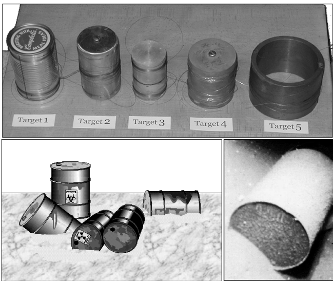
Fig.2 The targets used in these experiments (top) were scaled versions of those usually encountered in marine dumpsites, e.g. oil drums and radioactive waste (bottom).
