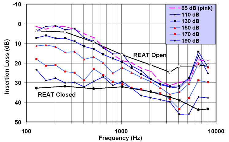
Fig. 4 – IL for the Combat Arms Earplug over an 80-dB range in impulse sound levels and for steady 85-dB pink noise as compared to REAT measurements for the open and closed orifices.
