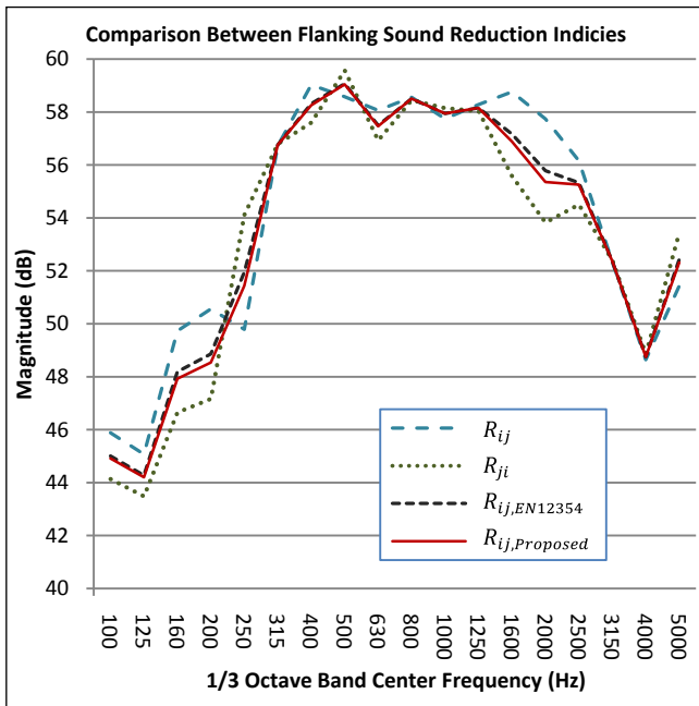
Fig.2 Comparison between R_{ij} , R_{ji} , R_{ij,Proposed} , and R_{ij,EN12354} for a lightweight, double-leaf constructions of gypsum board on metal studs. The elements both had critical frequencies in the 4000 Hz 1/3 octave band.
