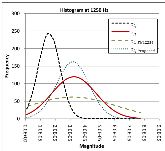
Fig.3 Comparison between the histograms of \tau_{ij} , \tau_{ji} , \tau_{ij,Proposed} and \tau_{ij,EN12354} .
