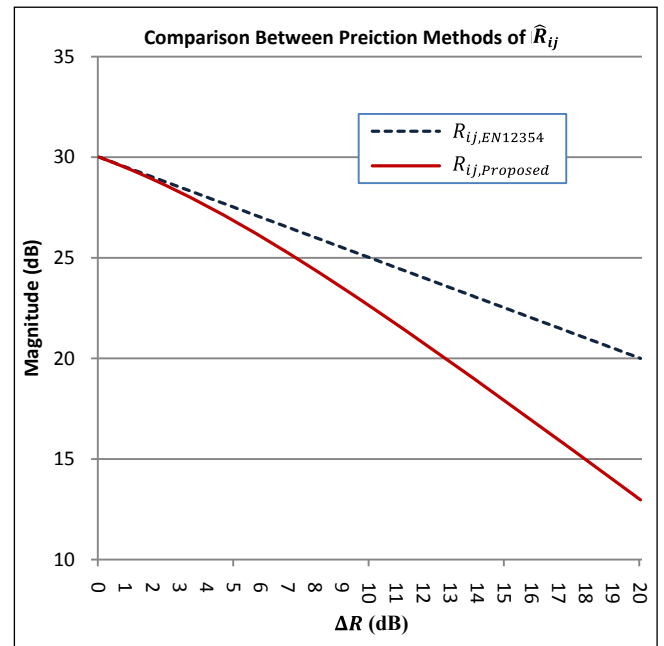
Fig.1 Comparison between R_{ij,Proposed} and R_{ij,EN12354} where R_{ij} = -10 \log \tau_{ij} and \Delta R = 10 \log \left( \frac{\tau_{ji}}{\tau_{ij}} \right) . The initial value of the calculations was set to R_{ij} = R_{ji} = 30\text{dB} .
